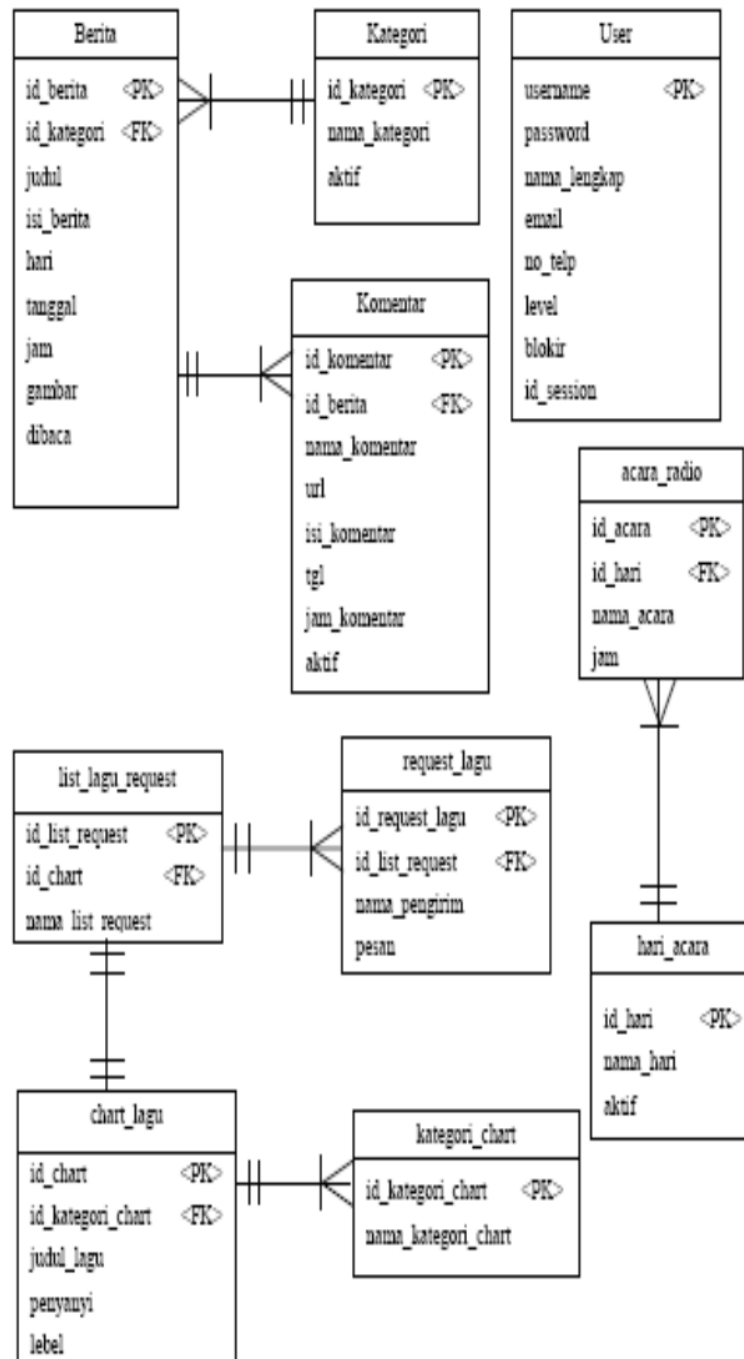
Gambar 5. Konseptual Database
