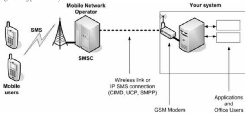
Gambar 1. Alur SMS Gateway
